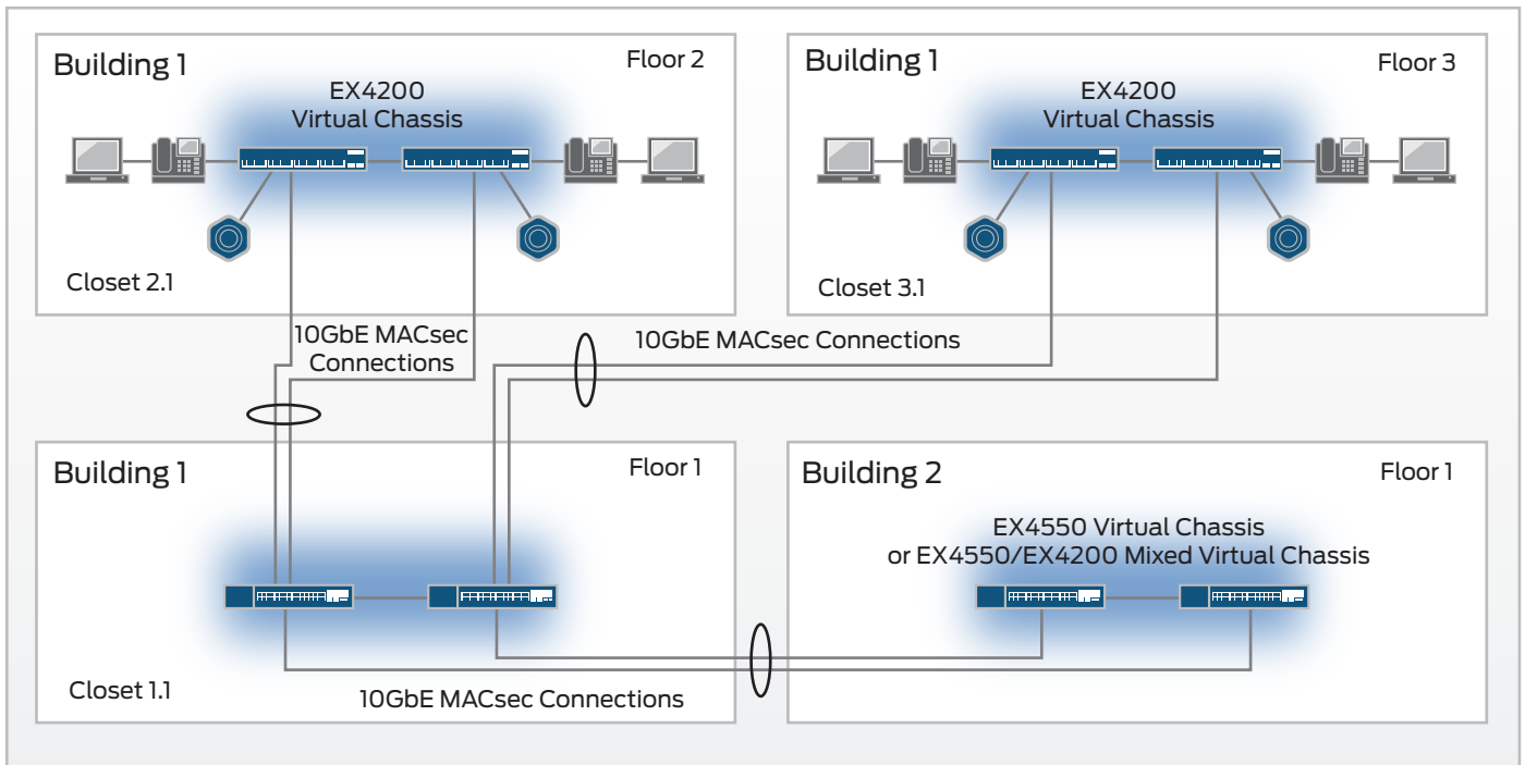
Figure 2: MACsec deployment with EX4200 and EX4550 switches.
