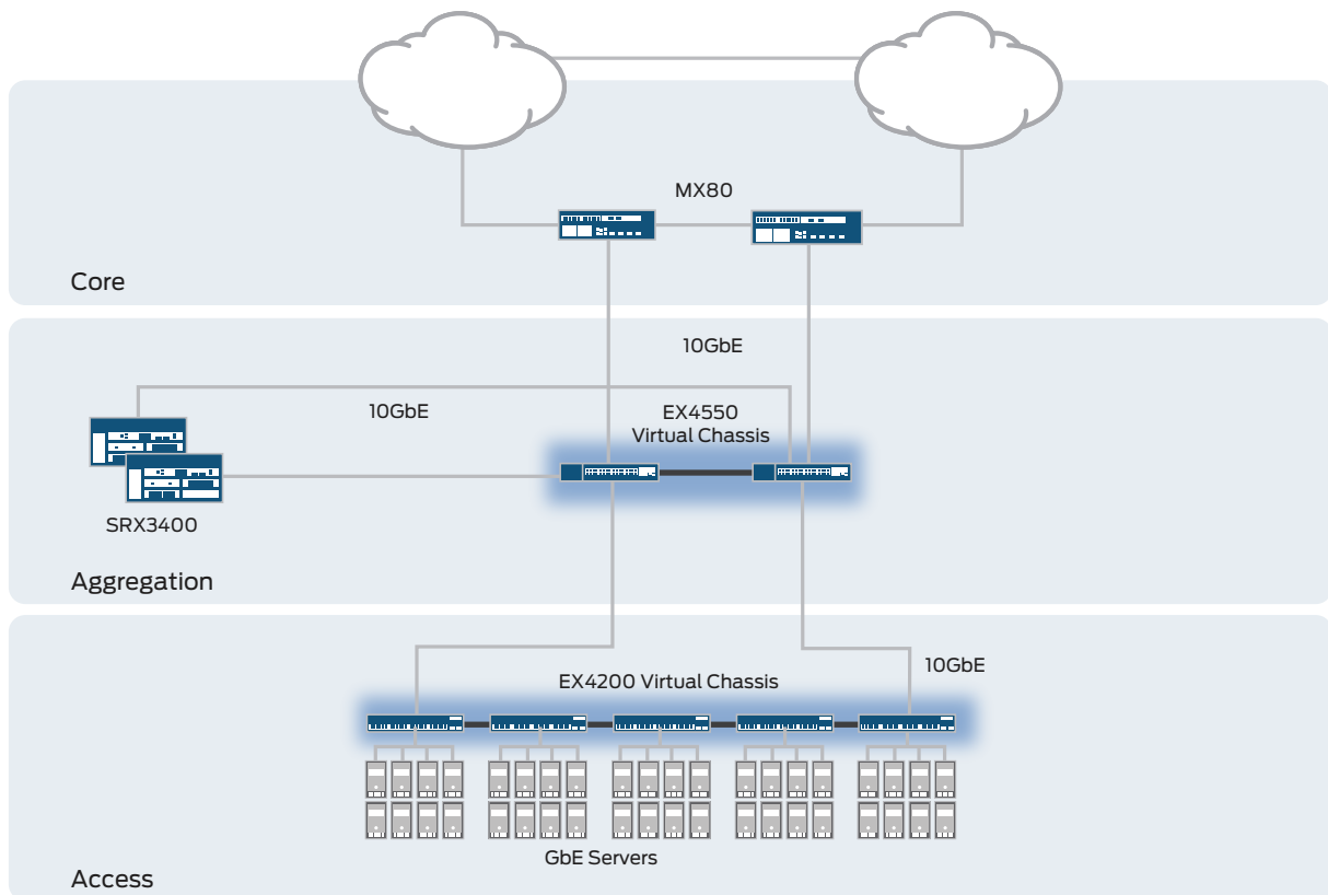
Figure 4: The EX4550 10GbE switch is ideal for small data center core deployments.
